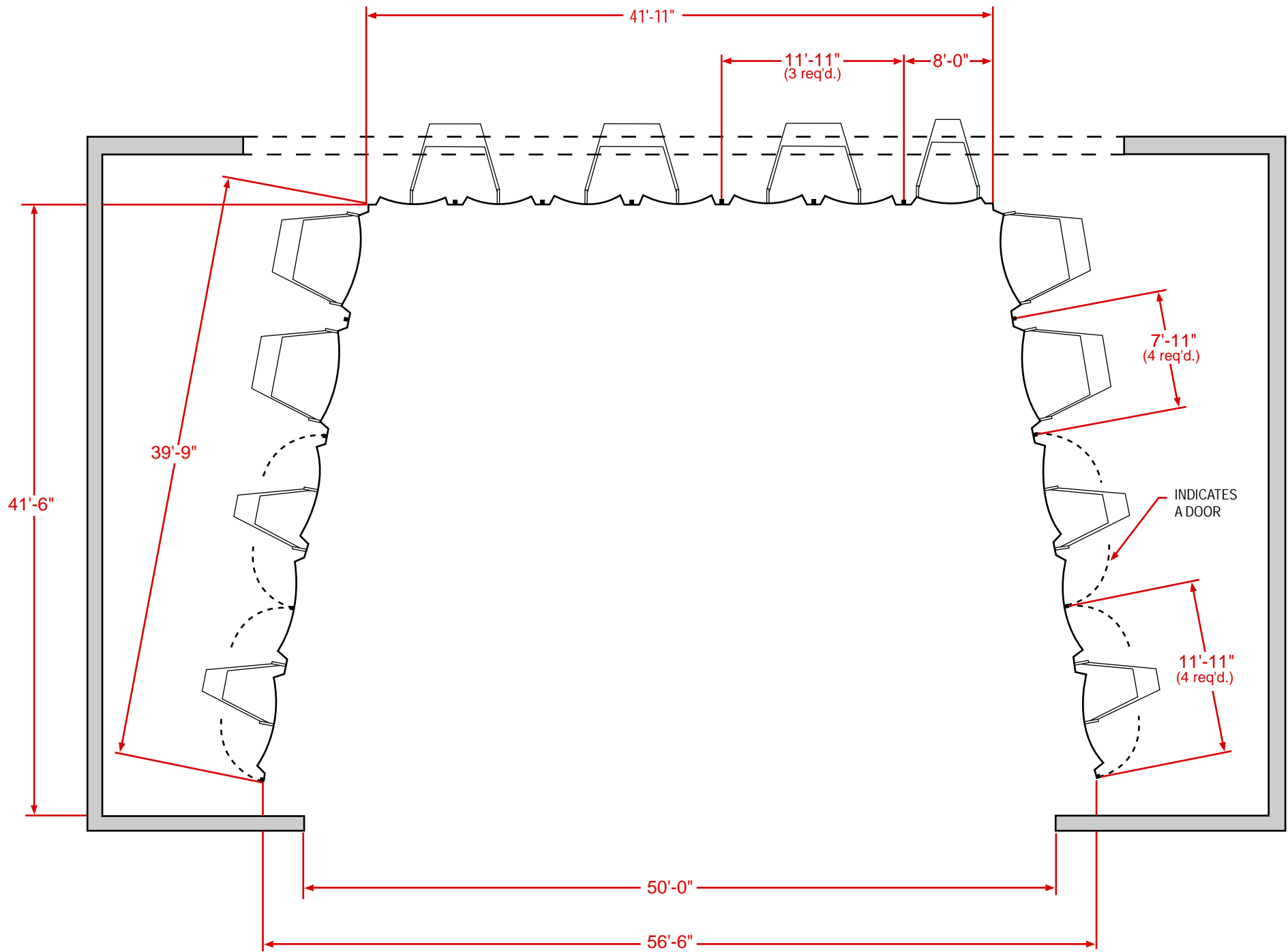
DESIGNER ORCHESTRA ENCLOSURE Blaisdell Concert Hall
